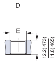
D: G drain port E: ISO 228/1 - G 1 /4
